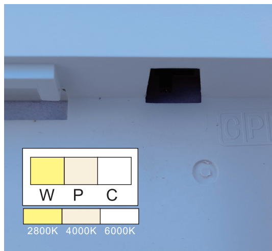
Select CCT by using the dip switch
