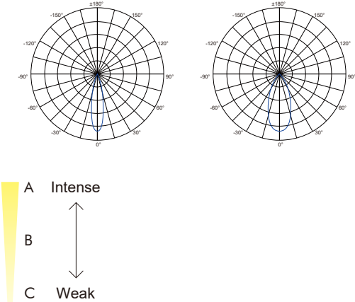
Photometric Information
